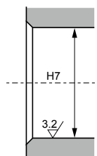
相配座孔 Mating Housing
